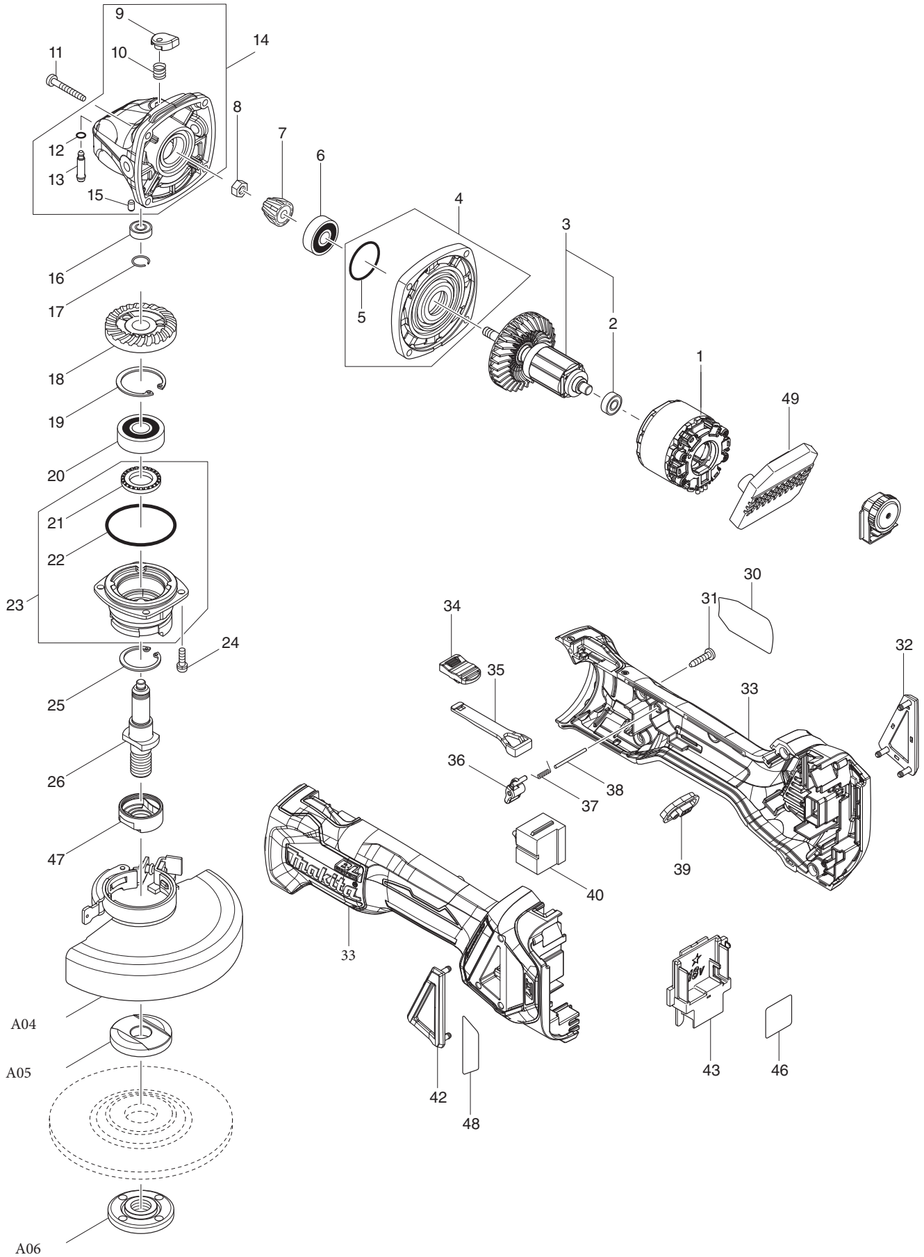
DGA513 - 18V LXT Brushless 5" Grinder, Slide Switch, w/ Brake, Variable Speed
